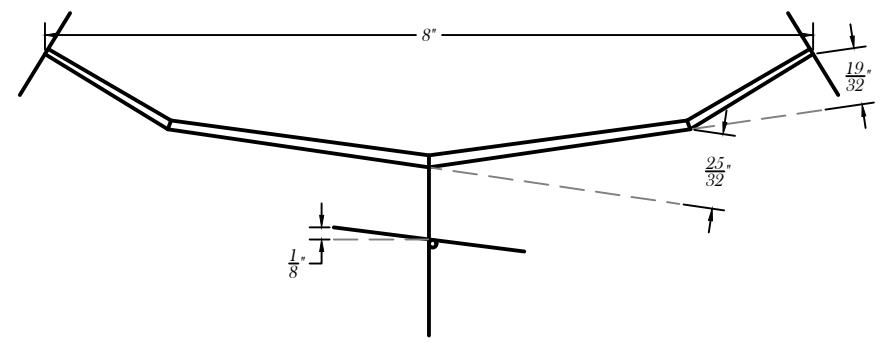
DIHEDRAL DETAIL (REAR VIEW) SCALE: 1:2
