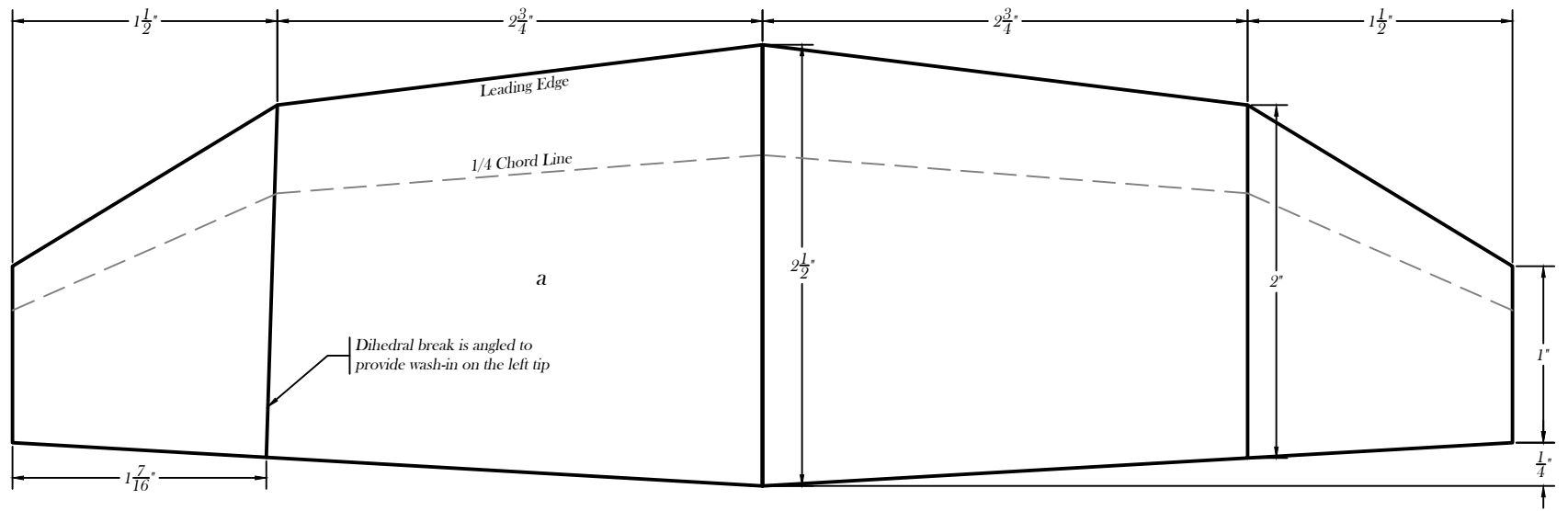
MAIN WING PLAN SCALE: 1:1
